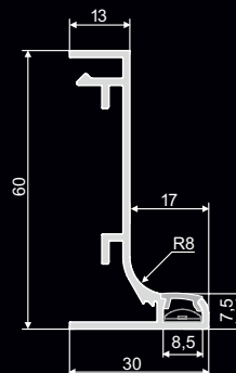
Listwa aluminiowa L – LED
