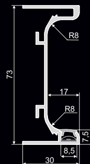
Listwa aluminiowa C – LED
